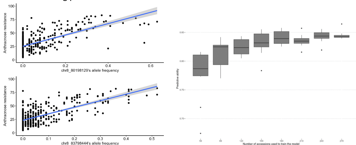
(Left) Percentage of resistance for anthracnose depending on the allele frequencies for the main two QTL. (Right) Predictive ability as a function of the number of accessions in the training population.
